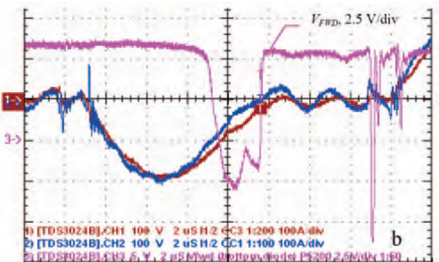
Fig. 11. Trace 3 - Forward drop of FWD IXYS DSEI 2x 61, two modules in parallel. a – high-bandwidth P6139A probe, b – differential probe. Both measurements taken with floating scope.
