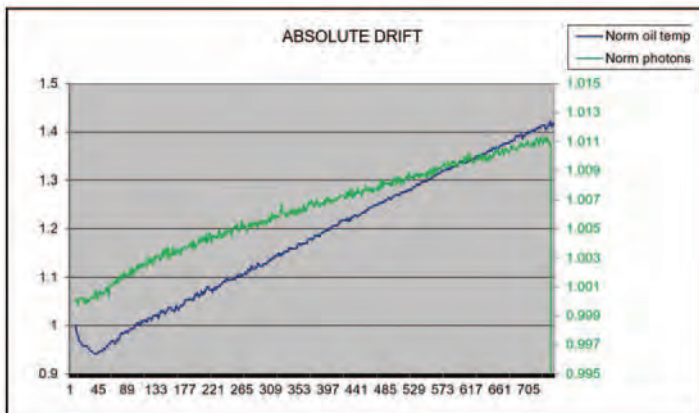
Figure 12: X-ray dose drift as a function of operating temperature. Horizontal axis shows time in seconds.
