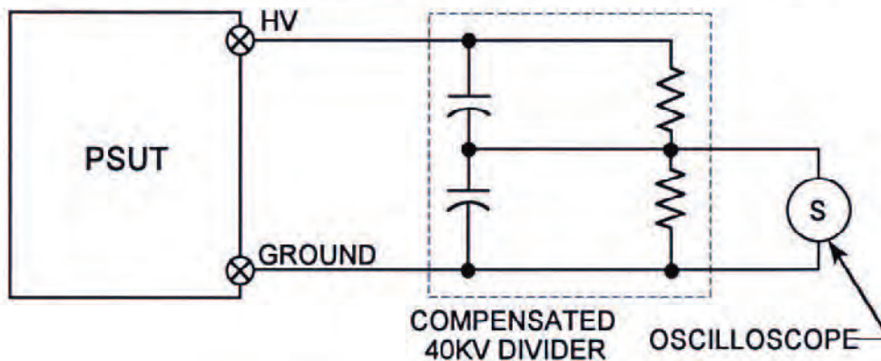
Figure 13 Ripple Measurement
