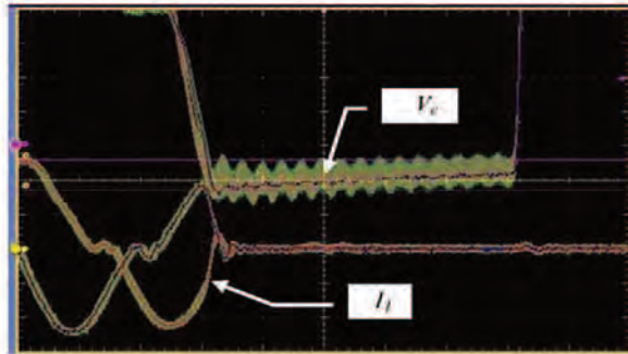
Fig. 19. Overlay of 600 frames ( V_c —100 V/div, 11–200 A/div) C_s = 33 nF, 10 kV at 1 kHz, V_r = 470 VUL. Horizontal 4 \mu s/div.
