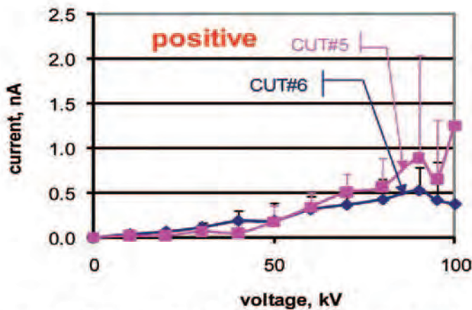
Figure 7. CUT#5, CUT#6. Leakage current at positive polarity.
