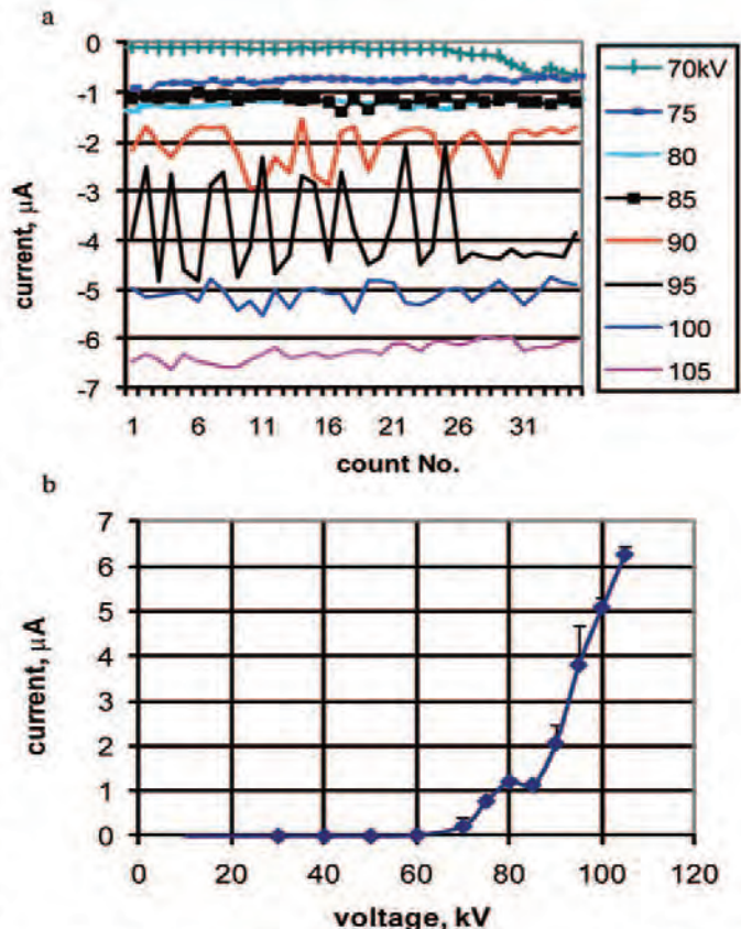
Figure 8. CUT#5. Leakage current (LC) at negative polarity. a) LC dependence on time (count number); b) LC as a function of applied voltage.
