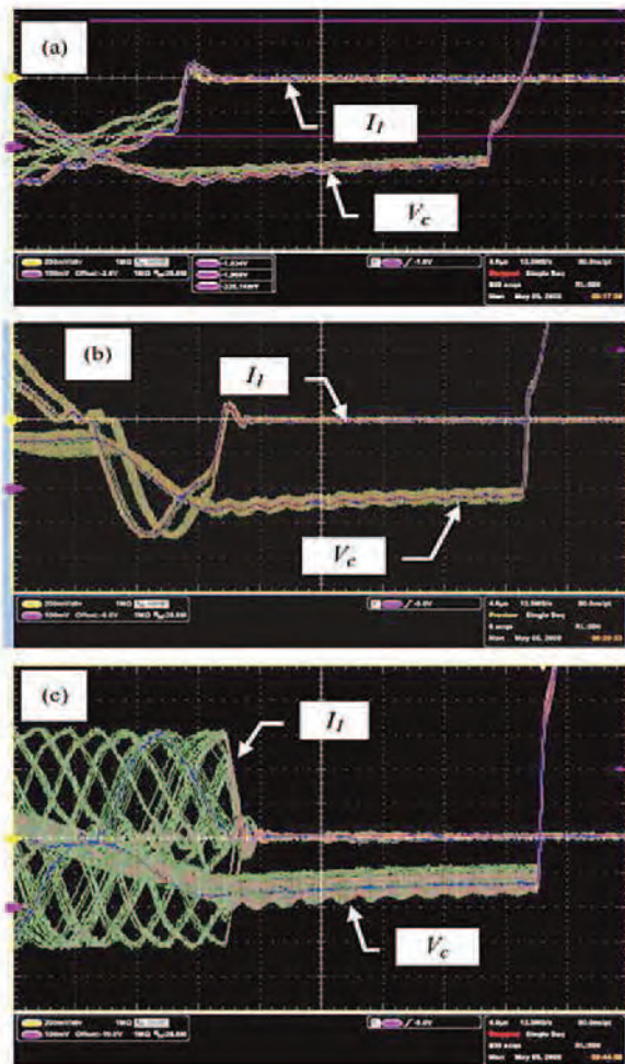
Fig. 15. Overlay of 80 frames ( V_c —100 V/div, I_t —100 A/div) for: (a) high line, 2 kV at 1 kHz; (b) nominal line, 6 kV at 1 kHz; and (c) high line, 10 kV at 1 kHz. Horizontal 4 \mu s/div.
