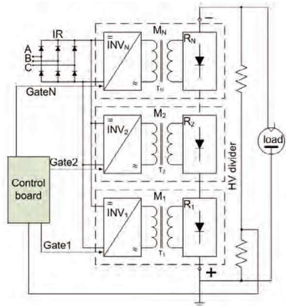
Fig. 1. HVPS block-diagram.
