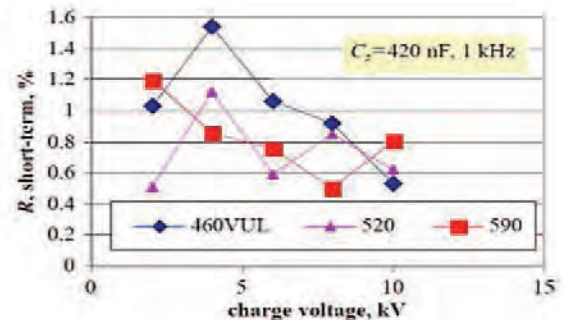
Fig. 16. Short-term repeatability.
