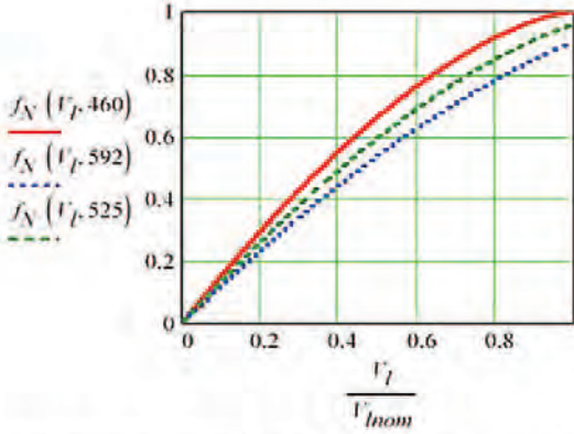
Fig. 3. ZOC curves for low (460 V), high (592 V), and normal (525 V) dc rail voltages. V_{nom} is nominal load voltage.
