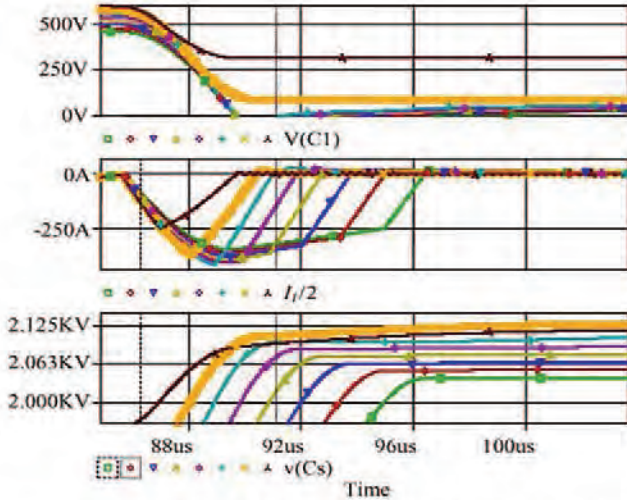
Fig. 7. Programmed charge voltage 2 kV. V_t = 460\text{ V}, 480\text{ V}, \dots, 600\text{ V} . C_s = 200\text{ nF} . Primary current I_1 is halved. Curves corresponding to largest overshoot are in thicker lines.
