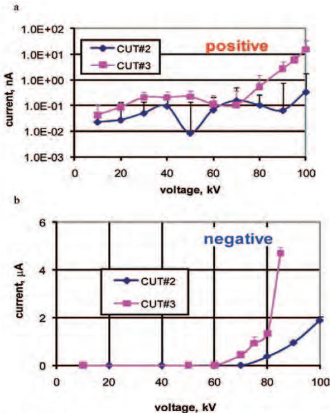
Figure 5. Leakage current as a function of applied voltage for CUT#2 [flush cut (FC), shrink tube (SHT), l = 20 cm polyethylene bared length] and CUT#3 (FC, SHT, l = 14.7 cm) at (a) positive and (b) negative polarity.
