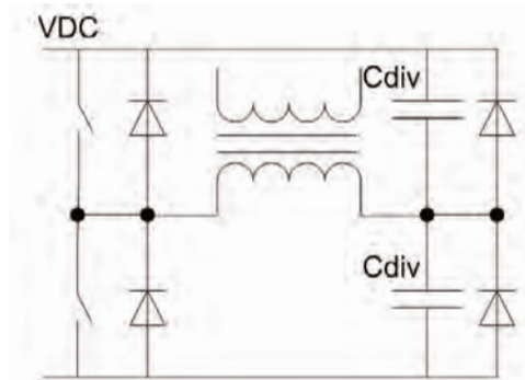
Fig. 2. Inverter with energy dosing capacitors
