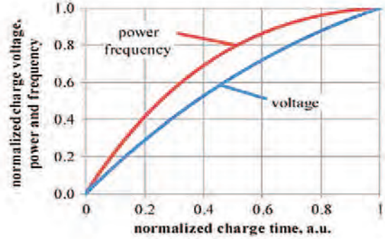
Fig. 4. Time dependence of load voltage, charging power, and frequency at ZOC.
