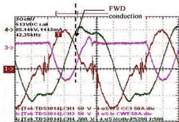
Fig. 4. Nominal line P = 28.7 kW (Trace 1) Primary winding current (halved). (Trace 3) Collector current (halved). (Trace 4) Voltage across resonant capacitors. FWD conducts to the right of the dotted line.
