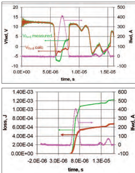
Fig. 9. FWD IXYS DSEI 2x61 losses. Plot a – green trace is measured signal; brown trace is V_{fwd} adjusted for inductive drop L di/dt (diode assembly inductance assessed at 5nH). Green and brown curves plot b match their counterparts in plot a. Divider Fig. 7, Floating scope.
