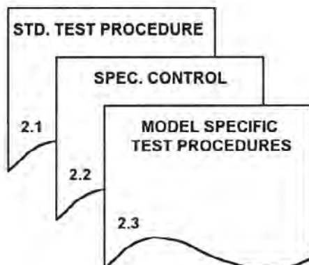
Figure 1. Document Organization
