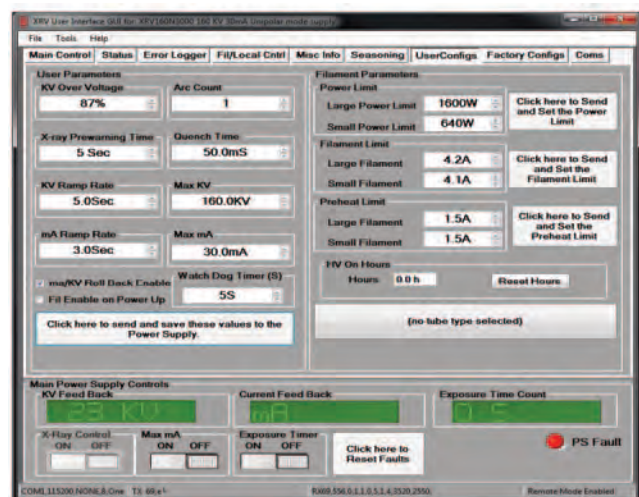
Figure 5a – GUI (Graphic User Interface) User Tube Configuration Screenshot
