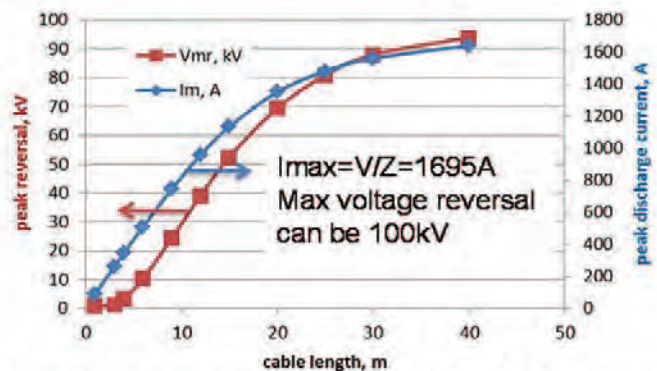
Figure 2. Dependence of peak reversal voltage and peak discharge current ( V(T1:A+) and IB(T1) , respectively, per notation of Figure 1) on cable length (referenced to charge voltage of 100 kV). In these simulations, TTRAN=1 \mu s (actual transition from 90% to 10% is 200ns).
